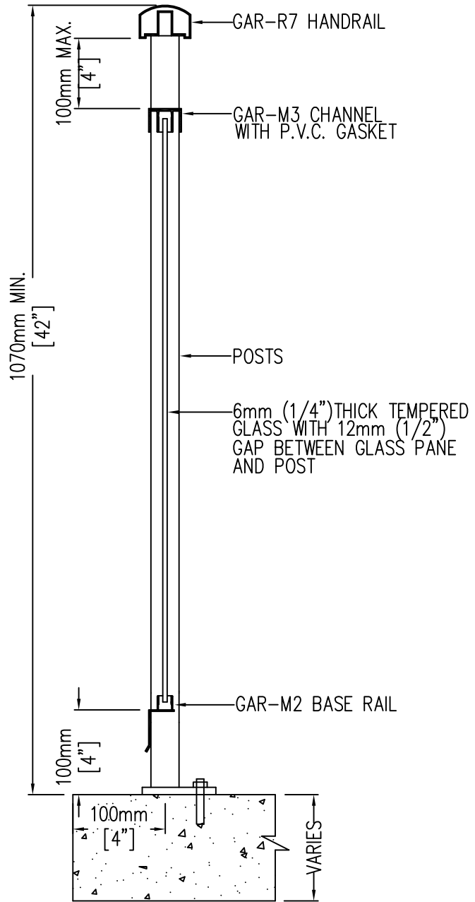
BALCONY GUARD SECTION
