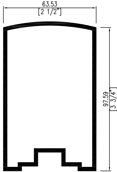
GAR-R2 TOP RAIL
