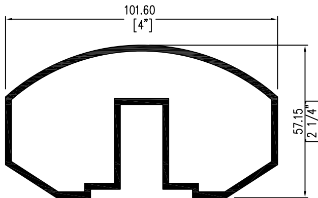
GAR-R4 TOP RAIL
