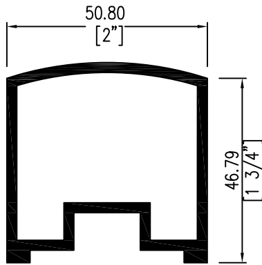
GAR-R1 TOP RAIL
